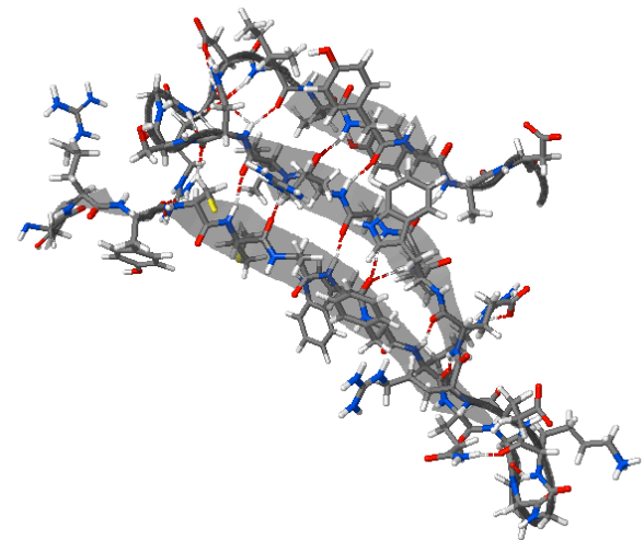
Hydrogen-bonding in beta-sheet
