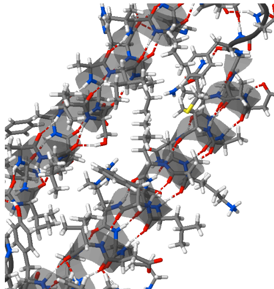
Hydrogen-bonding in alpha helix
